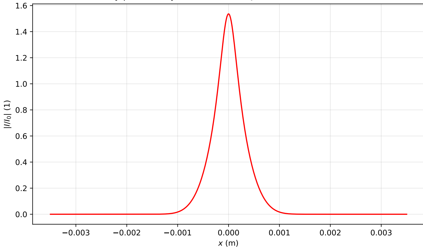
Intensity profile I(x, y = 0, z = 0.239)/I_0 , \text{Pin}=6.0\text{Pcr} , artificial time
